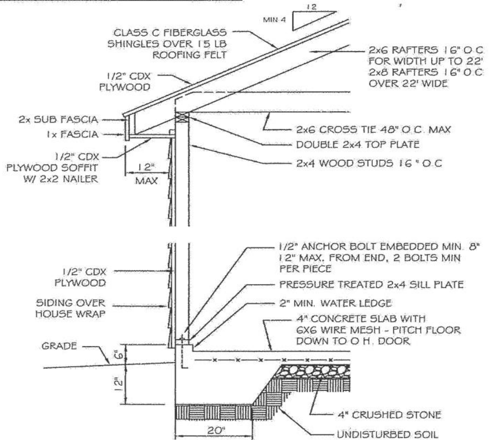
_____ WALL SECTION
